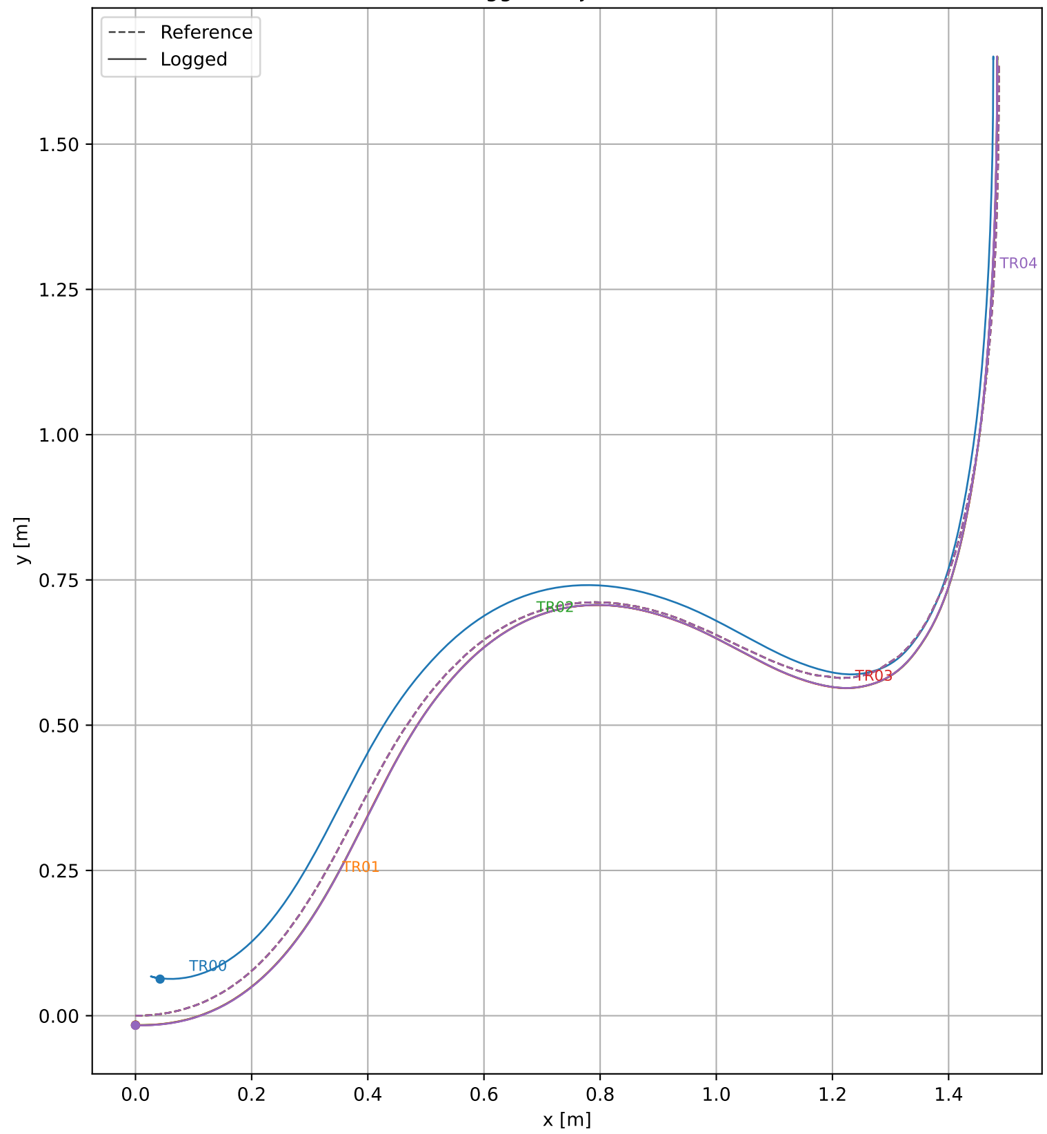
Logged Trajectories
